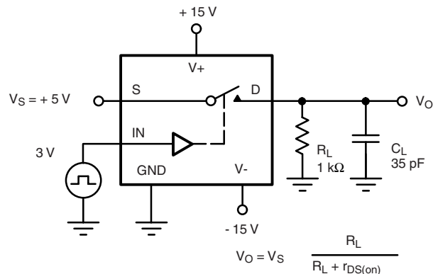
Figure 2. Switching Time
