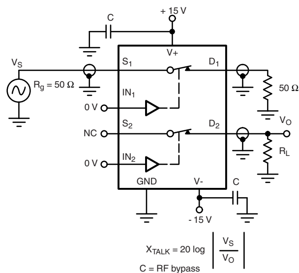
Figure 5. Channel-to-Channel Crosstalk
