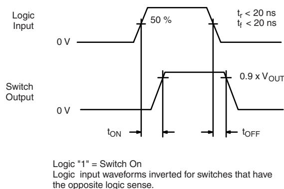
Figure 1. Switching Time
