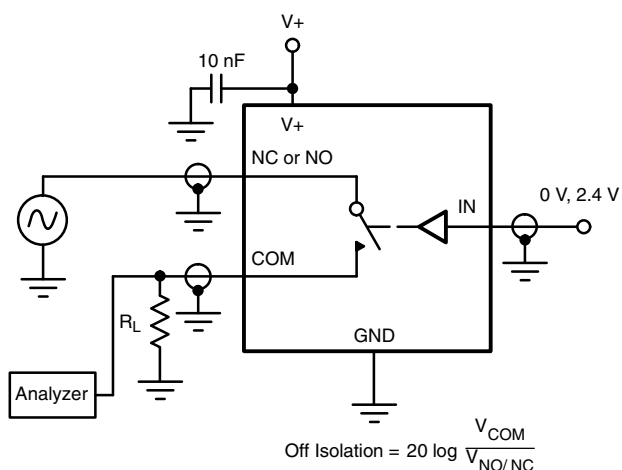
Figure 3. Off-Isolation
