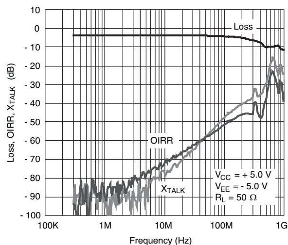
DG4051A Insertion Loss, Off-Isolation, Crosstalk vs. Frequency at \pm 5 \text{ V} Supply
