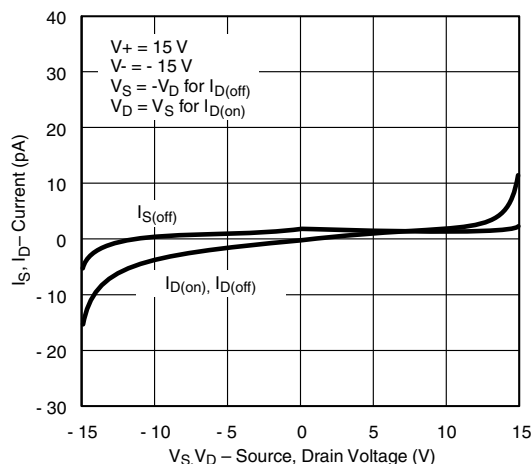
I_D , I_S Leakage Currents vs. Analog Voltage
