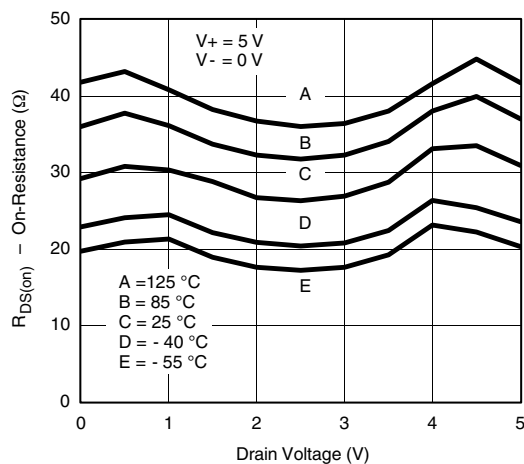
R_{DS(on)} vs. Drain Voltage and Temperature (Single Supply)
