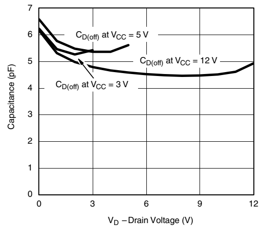
Drain Capacitance vs. Drain Voltage (Single Supply)
