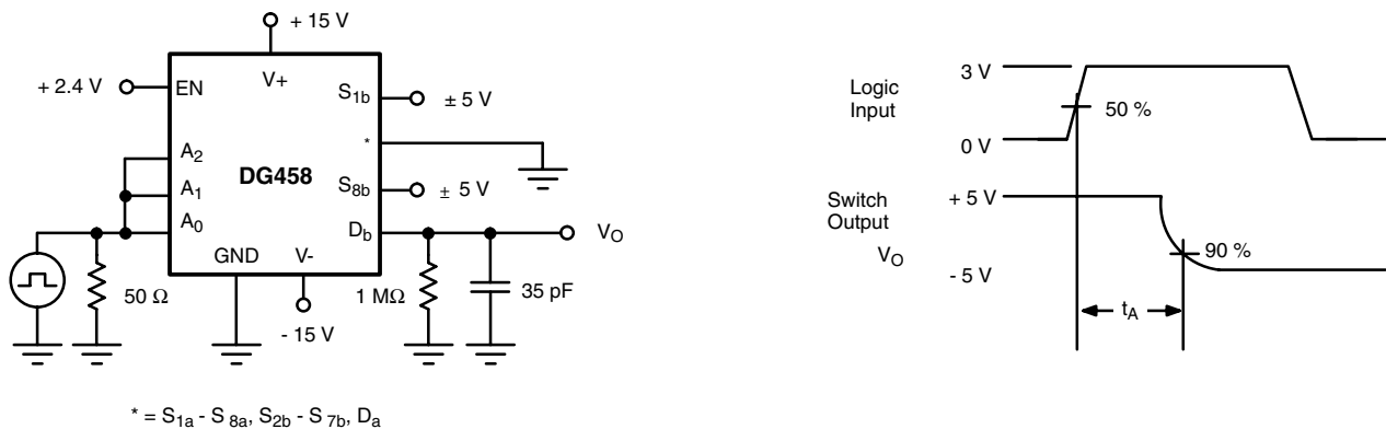
Figure 3. Transition Time
