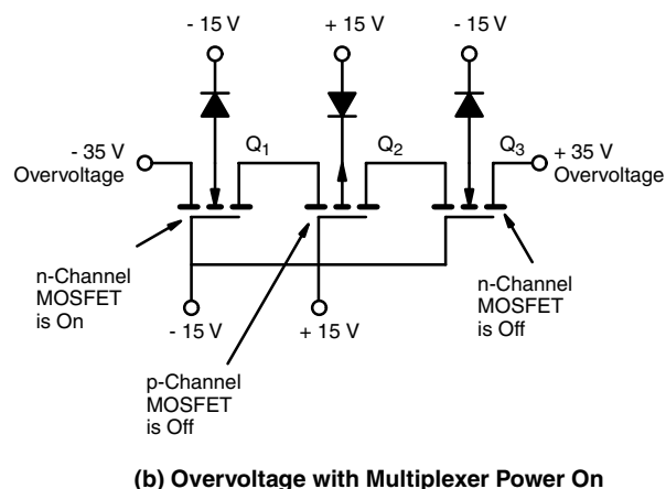
Figure 5. Overvoltage Protection
