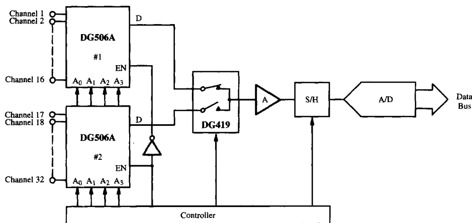
Figure 6. A 32-Channel Data Acquisition System
