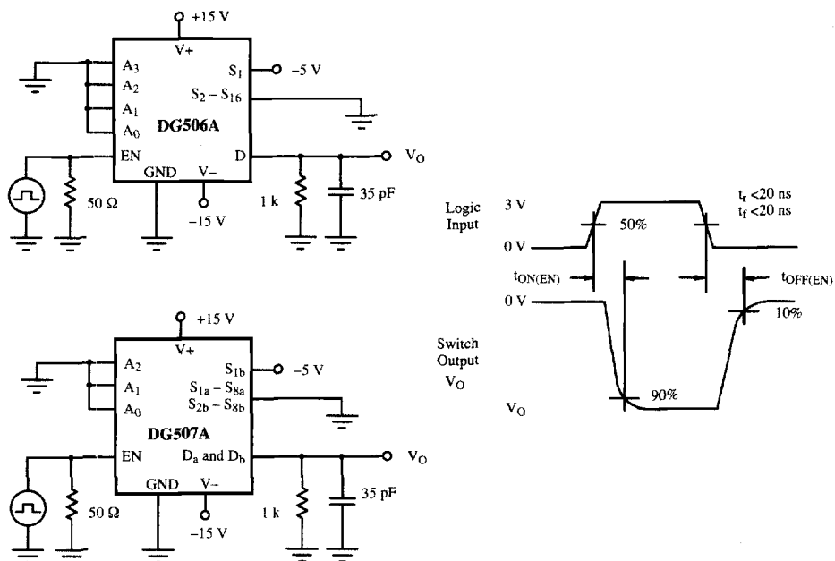
Figure 3. Enable Switching Time
