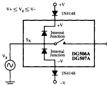
Figure 5. Overvoltage Protection Using Blocking Diodes
