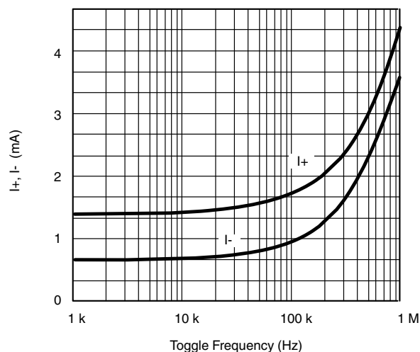
Supply Currents vs. Toggle Frequency
