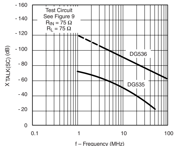
Single Channel Crosstalk vs. Frequency
