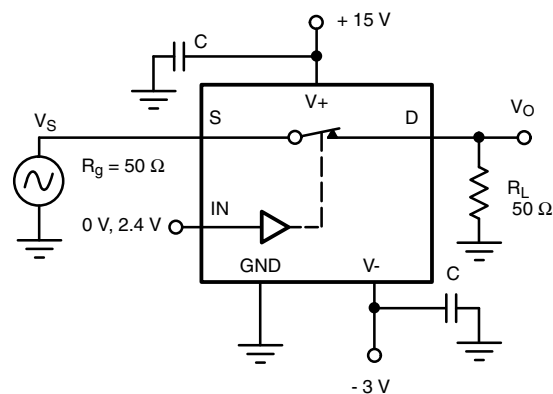
Figure 5. Bandwidth
