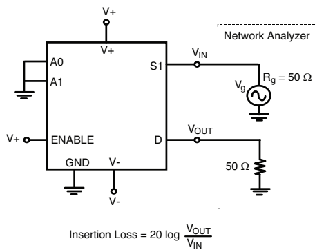
Figure 5. Insertion Loss
