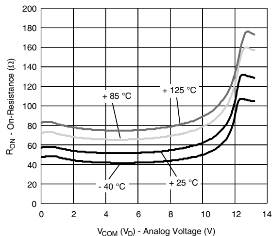
On-Resistance vs. Temperature (Single Supply)
