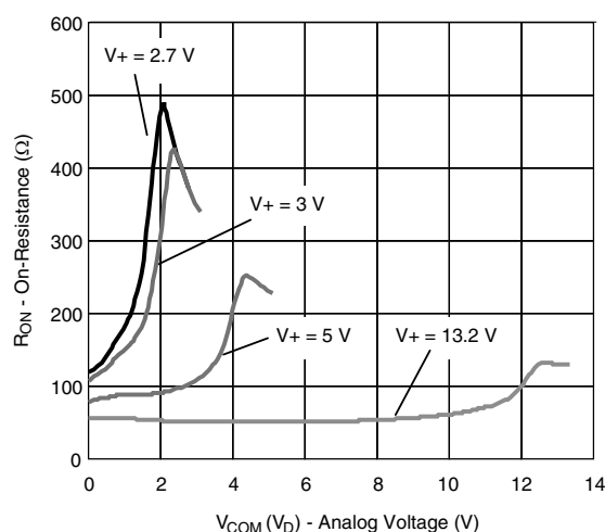
On-Resistance vs. V_D (Single Supply)
