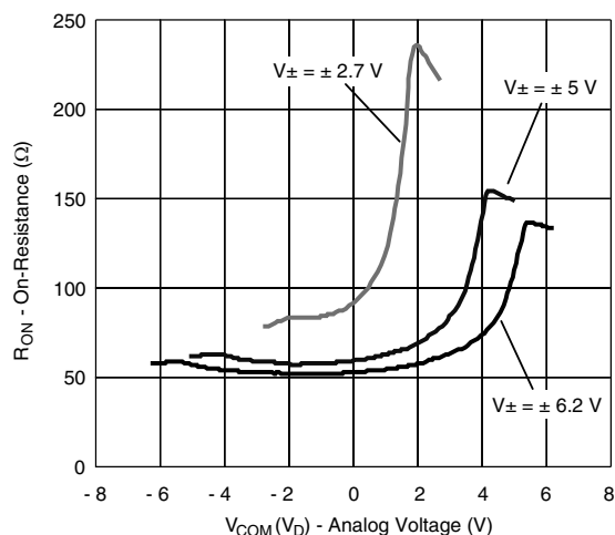
On-Resistance vs. V_D (Dual Supply)
