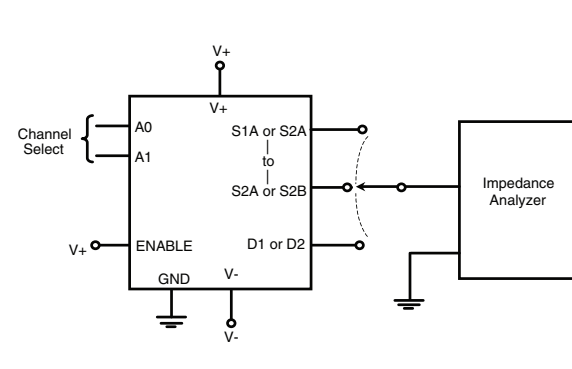
Fig. 8 - Source / Drain Capacitance
