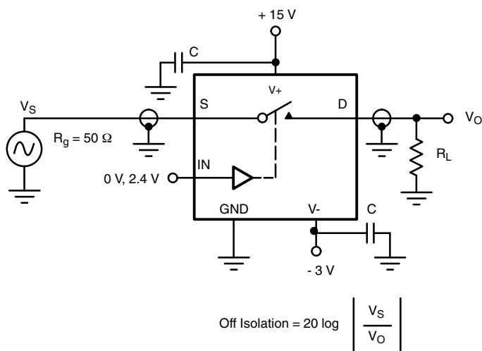
Figure 4. Off Isolation
