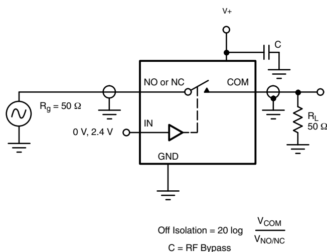
Figure 7. Off Isolation
