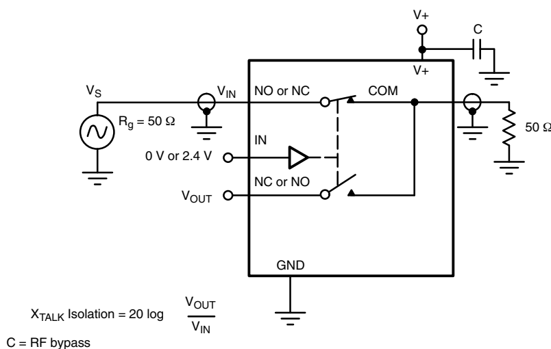
Figure 6. Crosstalk
