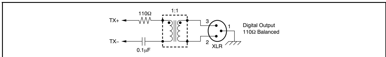
Figure 30. Transformer-Coupled Balanced Output Interface
