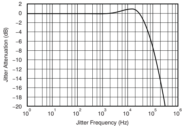
Figure 14. DIR Jitter Attenuation Characteristics
