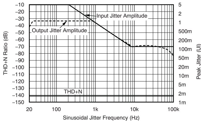
Figure 15. DIR Jitter Tolerance Plot
