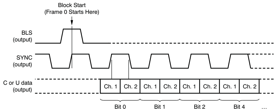
Figure 16. DIR Channel Status and User Data Serial Output Format Via the GPO Pins
