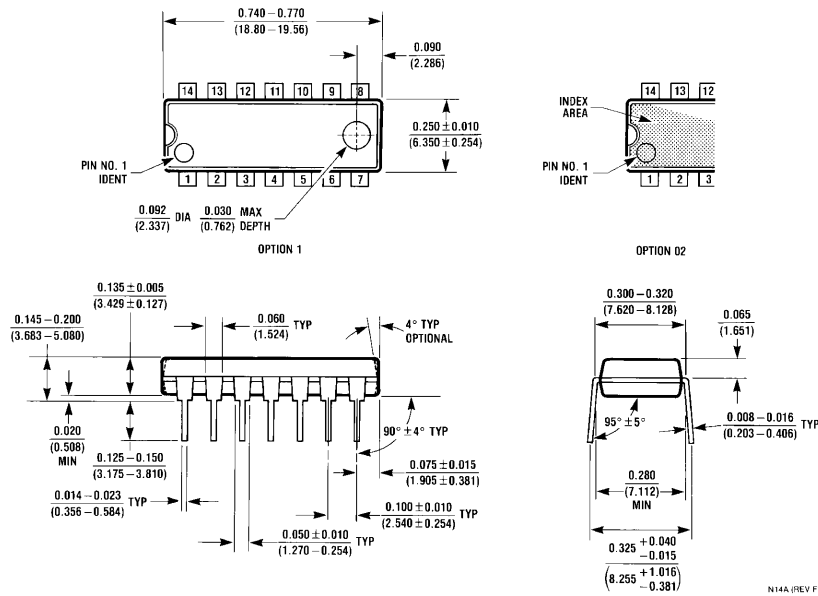
14-Lead Molded Dual-In-Line Package (N) Order Number DM7405N NS Package Number N14A
