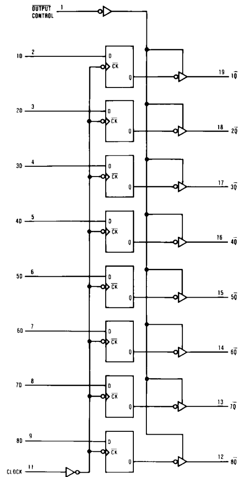
Logic Diagram
