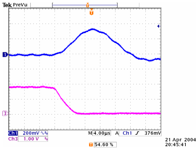
Figure 25: Typical transient response to step load change at 2.5A/μs from 100% to 50% of I_o , max at 3.3Vin, 1.8Vout (Cout = 1μF ceramic, 10μF tantalum)
