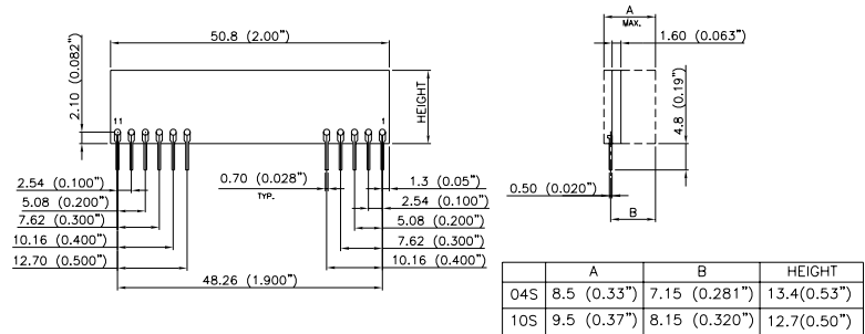
BACK VIEW
