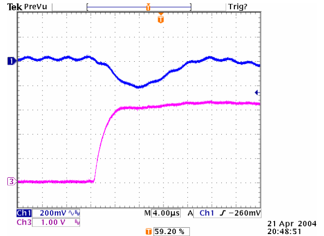
Figure 20: Typical transient response to step load change at 2.5A/\mu S from 50% to 100% of I_o , max at 5Vin, 3.3Vout (Cout = 1uF ceramic, 10μF tantalum)
