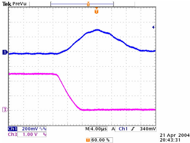
Figure 23: Typical transient response to step load change at 2.5A/μs from 100% to 50% of I_o , max at 3.3Vin, 2.5Vout (Cout = 1μF ceramic, 10μF tantalum)
