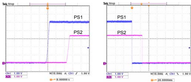
Figure 27: Sequential start-up
