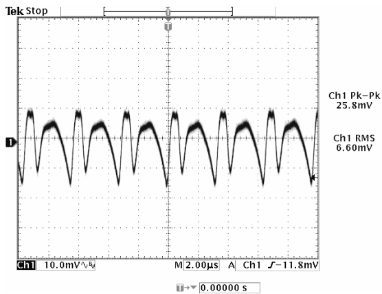
Figure 8: Output ripple & noise at 12Vin, 2.5V/10A out
