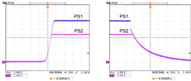
Figure 27: Sequential start-up
