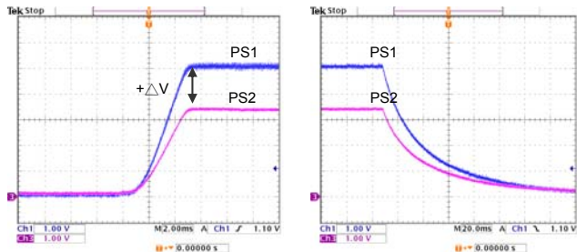
Figure 28: Simultaneous
