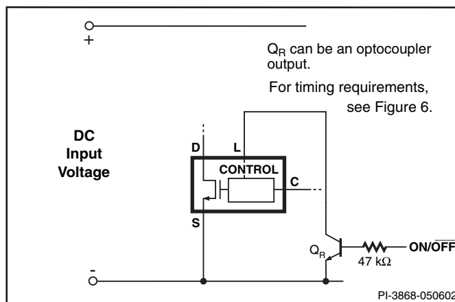
Figure 24. Synchronization.
