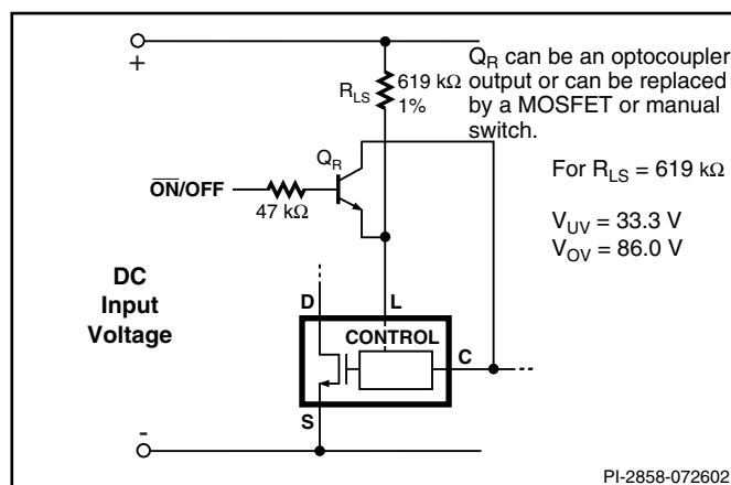
Figure 22. Active-off Remote ON/OFF with LINE-SENSE.
