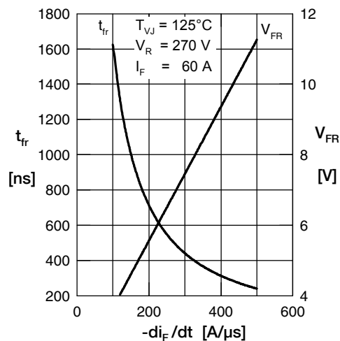
Fig. 6 Typ. forward recovery voltage V_{FR} & reco. time t_{fr} vs. di_F/dt
