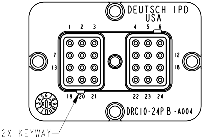
DRC10-24PB-A004 KEY -B-
