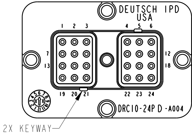
DRC10-24PD-A004 KEY -D-
