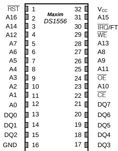
Encapsulated DIP
