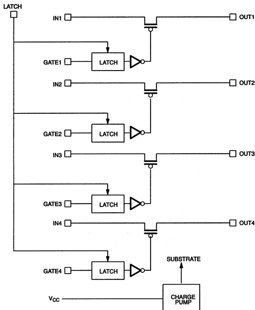
DS1640 BLOCK DIAGRAM Figure 1
