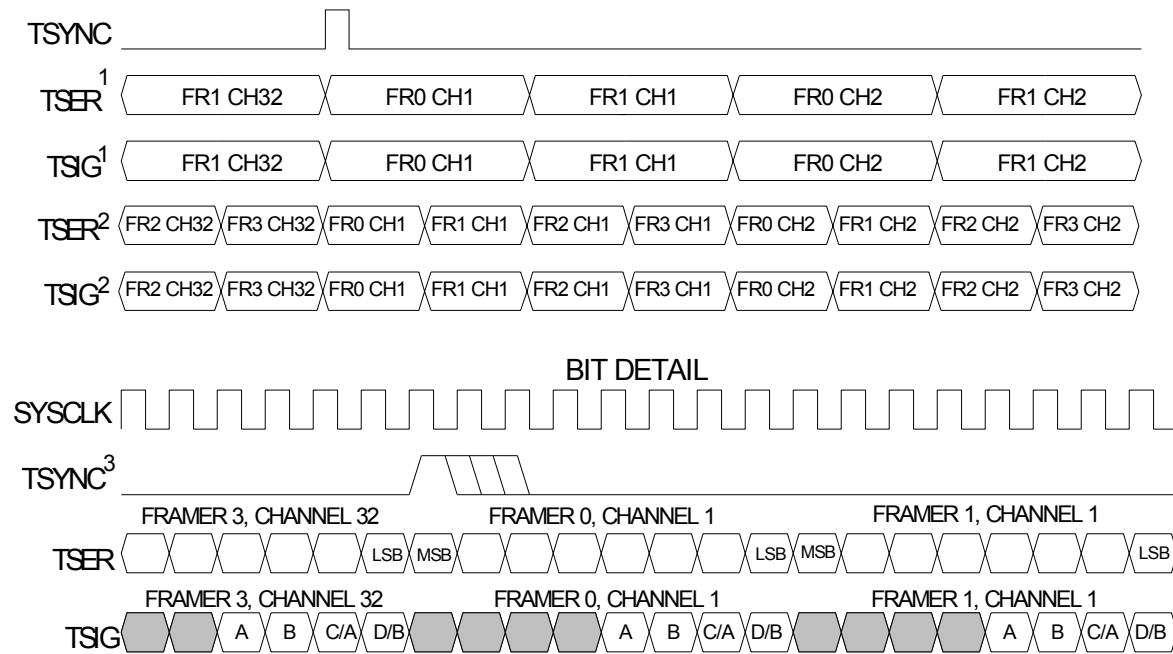
Figure 18-11. Transmit-Side Interleave Bus Operation, Byte Mode
