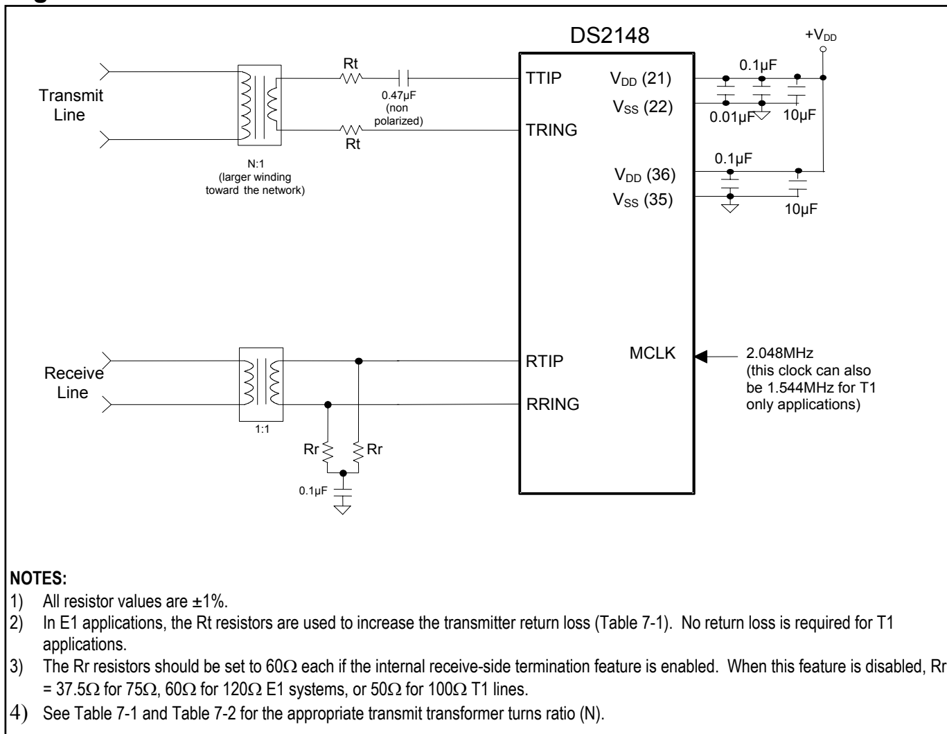
Figure 7-1. Basic Interface
