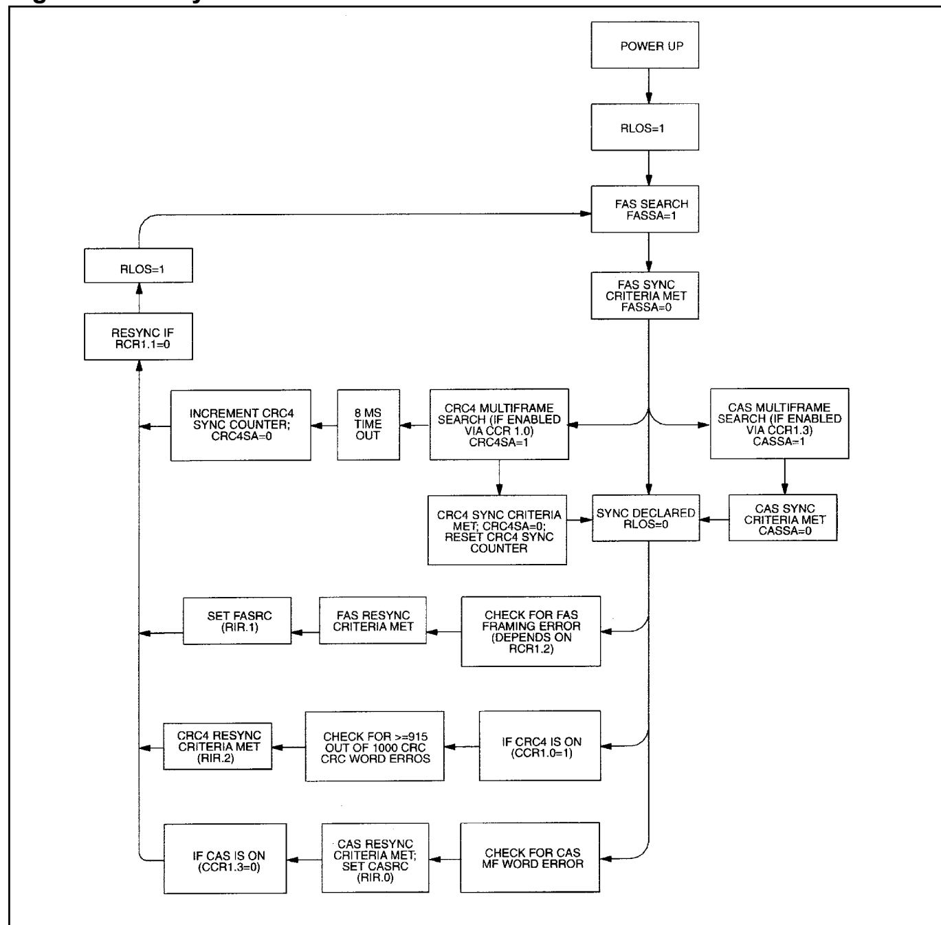
Figure 14-10. Synchronization Flow Chart
