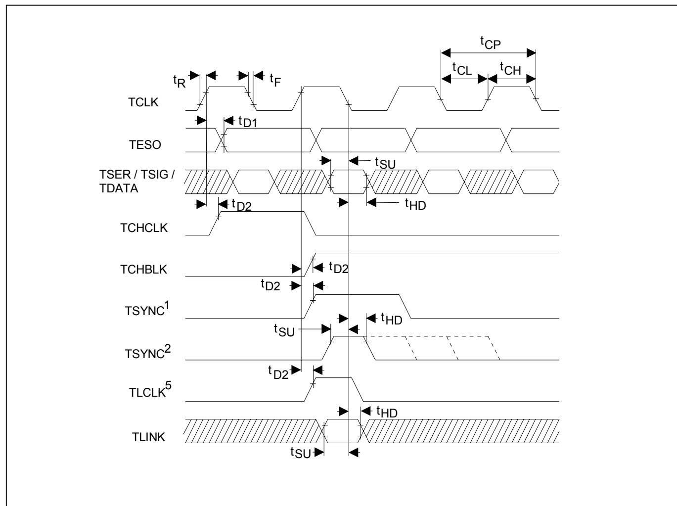
Figure 37-12. Transmit-Side Timing
