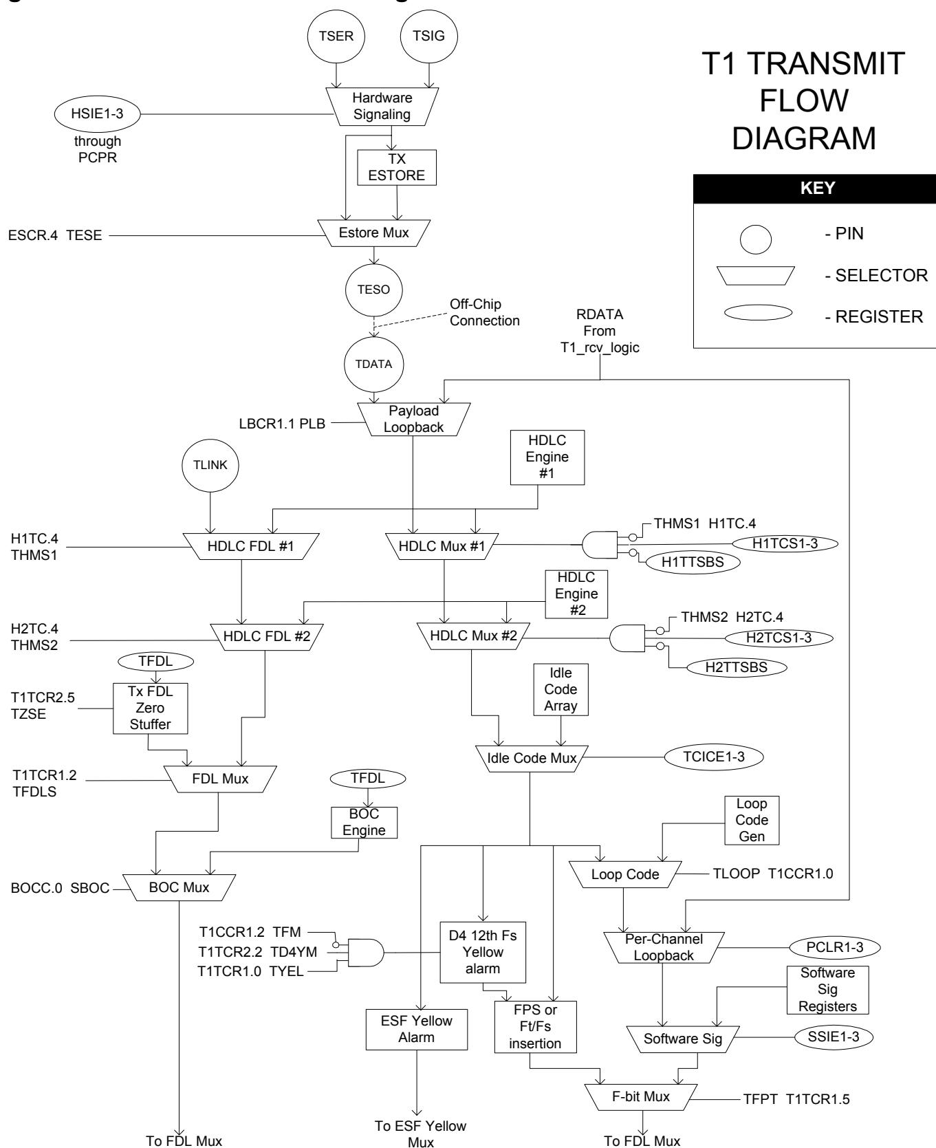
Figure 33-1. T1 Transmit Flow Diagram
