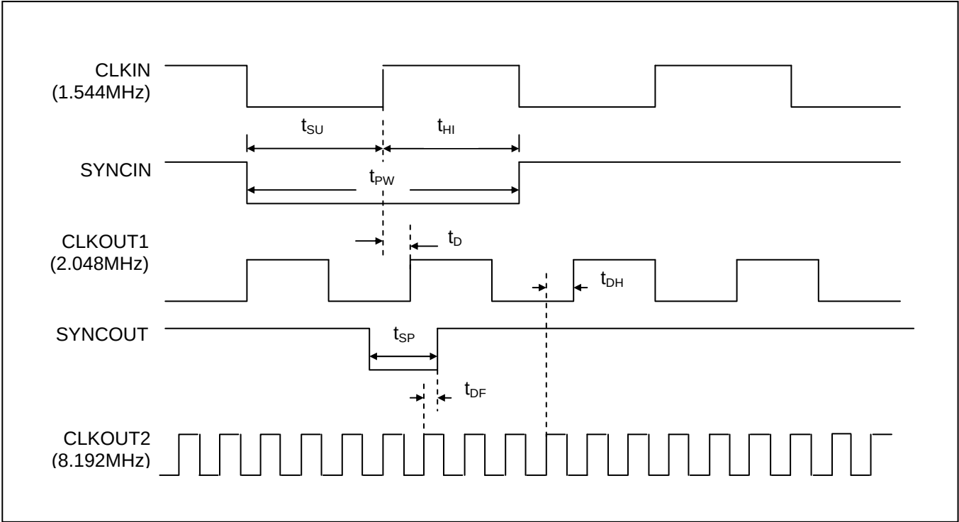
Figure 4-5. DS21604 Low-to-High Frequency Conversion Frame-Sync Alignment
