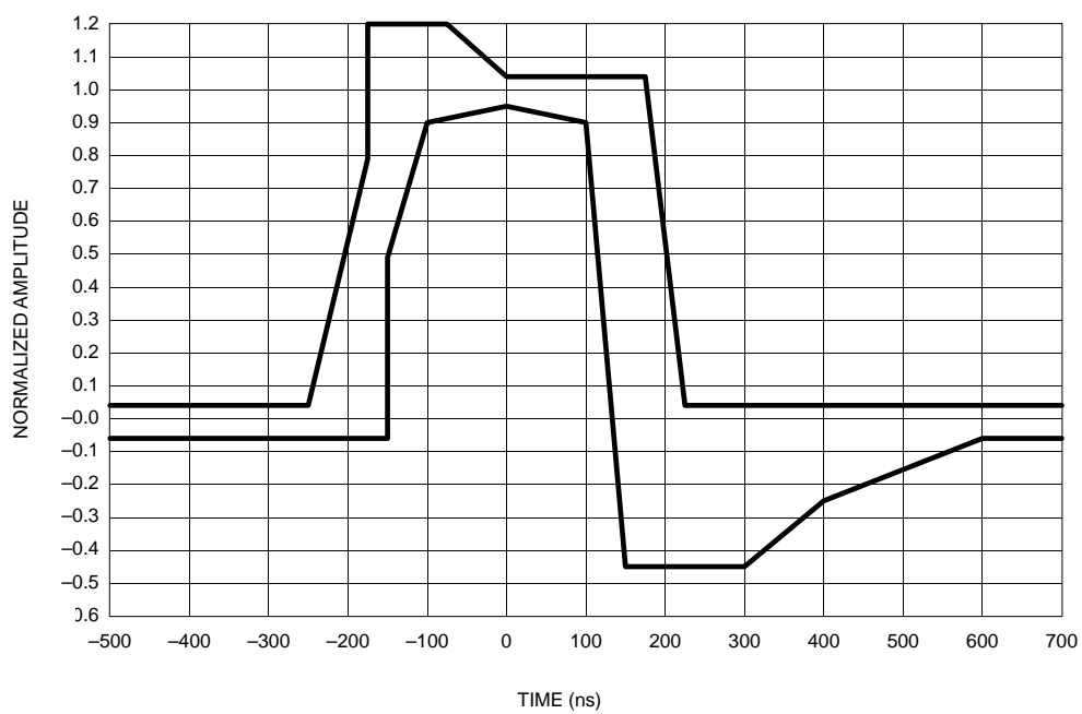
OUTPUT PULSE TEMPLATE Figure 3
