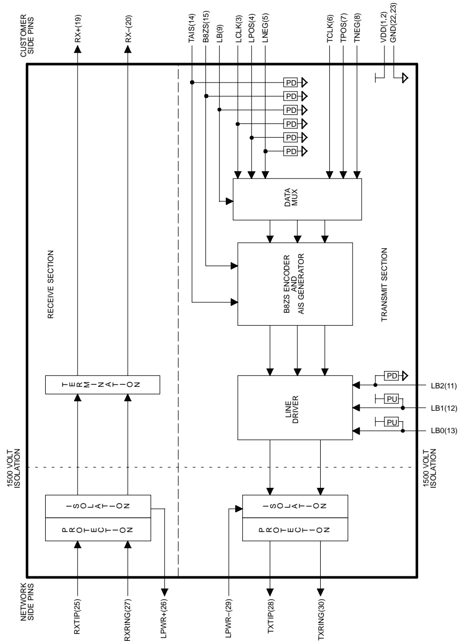
DS2290 BLOCK DIAGRAM Figure 1
