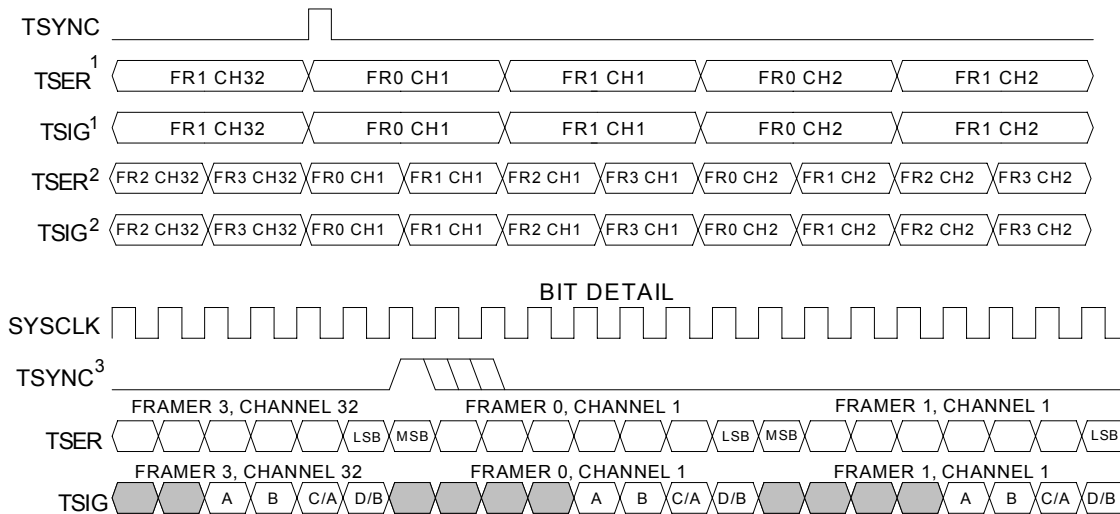
Figure 13-13. T1 Transmit-Side Interleave Bus Operation, BYTE Mode
