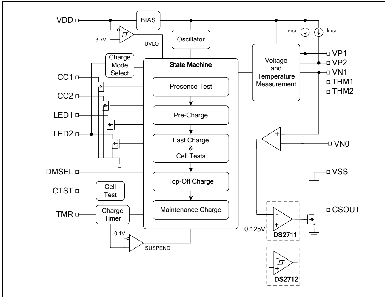
Figure 1. Block Diagram
