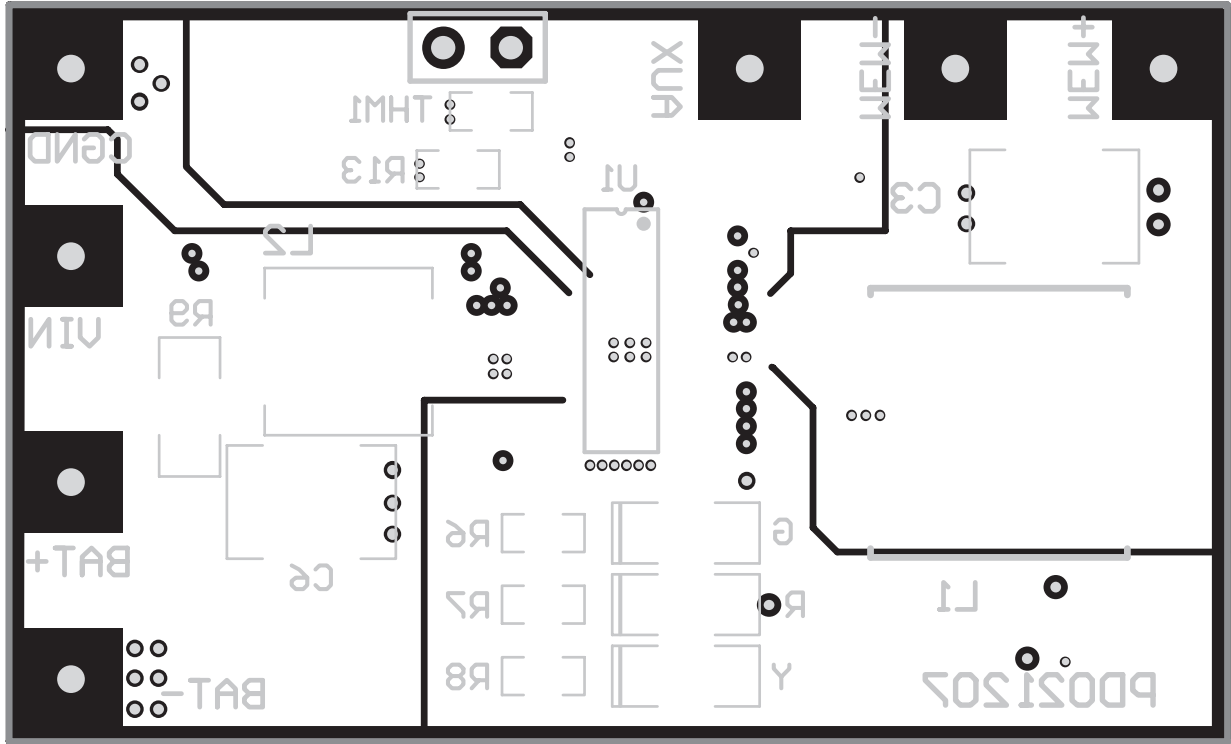
Figure 5. DS2731 EV Kit Board—Middle Layer
