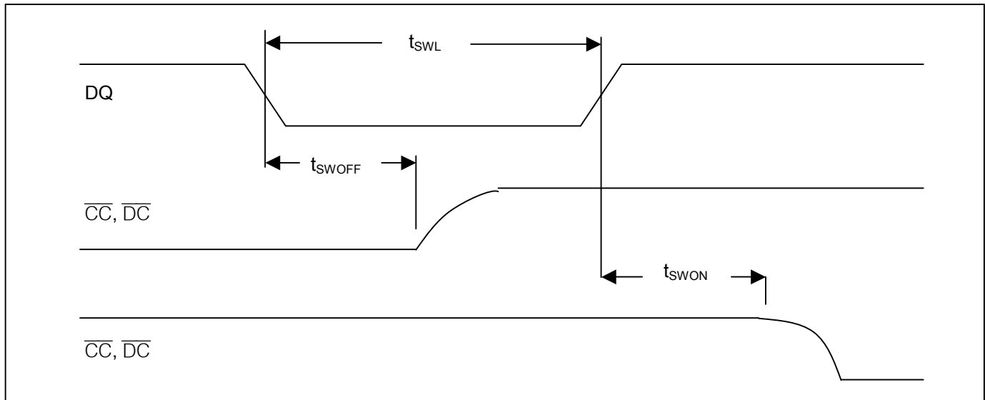
Figure 20. Swap Command Timing
