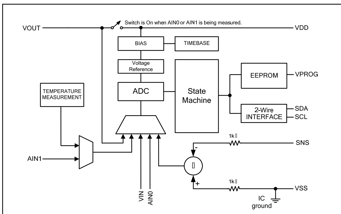
Figure 2. Block Diagram
