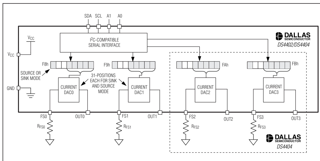
Figure 1. Functional Diagram
