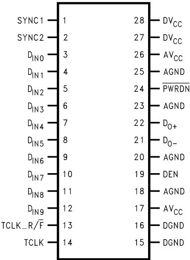
DS92LV1023EMQ - Serializer
