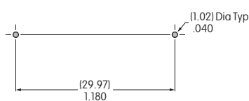
PCB Footprint
