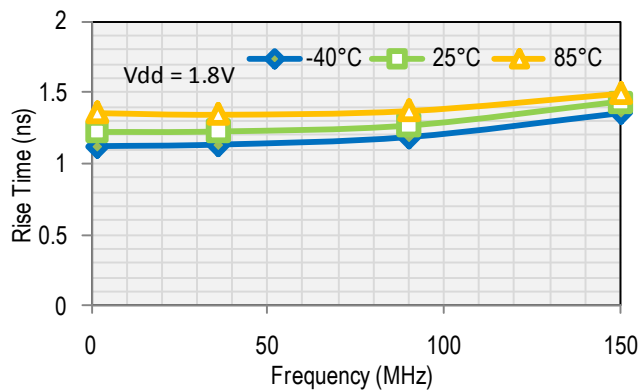
Rise Time
