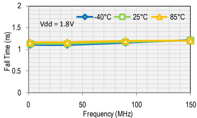
Fall Time
