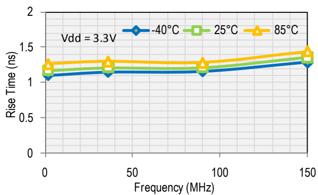
Rise Time
