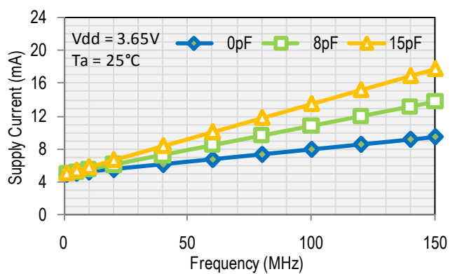
Supply Current
