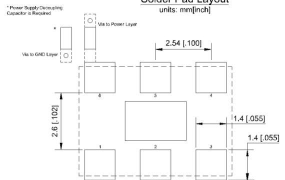
Recommended Solder Pad Layout units: mm[inch]
