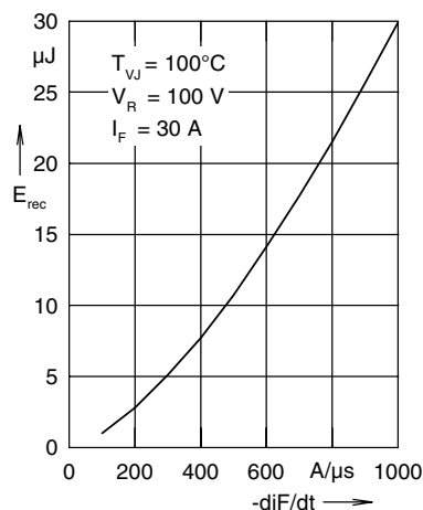
Fig.7 Recovery energy E_{rec} versus -di_F/dt
