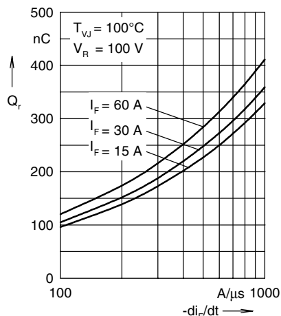
Fig.2 Reverse recovery charge Q_{rr} versus -di_F/dt
