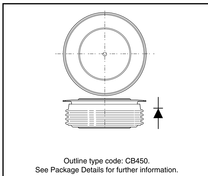
Fig. 1 Package outline
