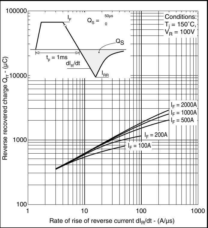
Fig.5 Recovered charge
