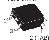
TO-268 AA Version AT
