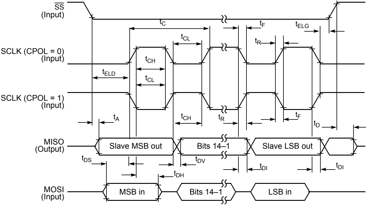
Figure 3-22 SPI Slave Timing (CPHA = 0)
