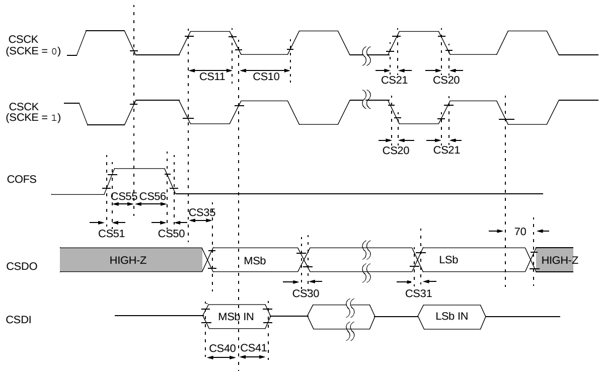
FIGURE 23-12: DCI MODULE (MULTICHANNEL, I 2 S MODES) TIMING CHARACTERISTICS
