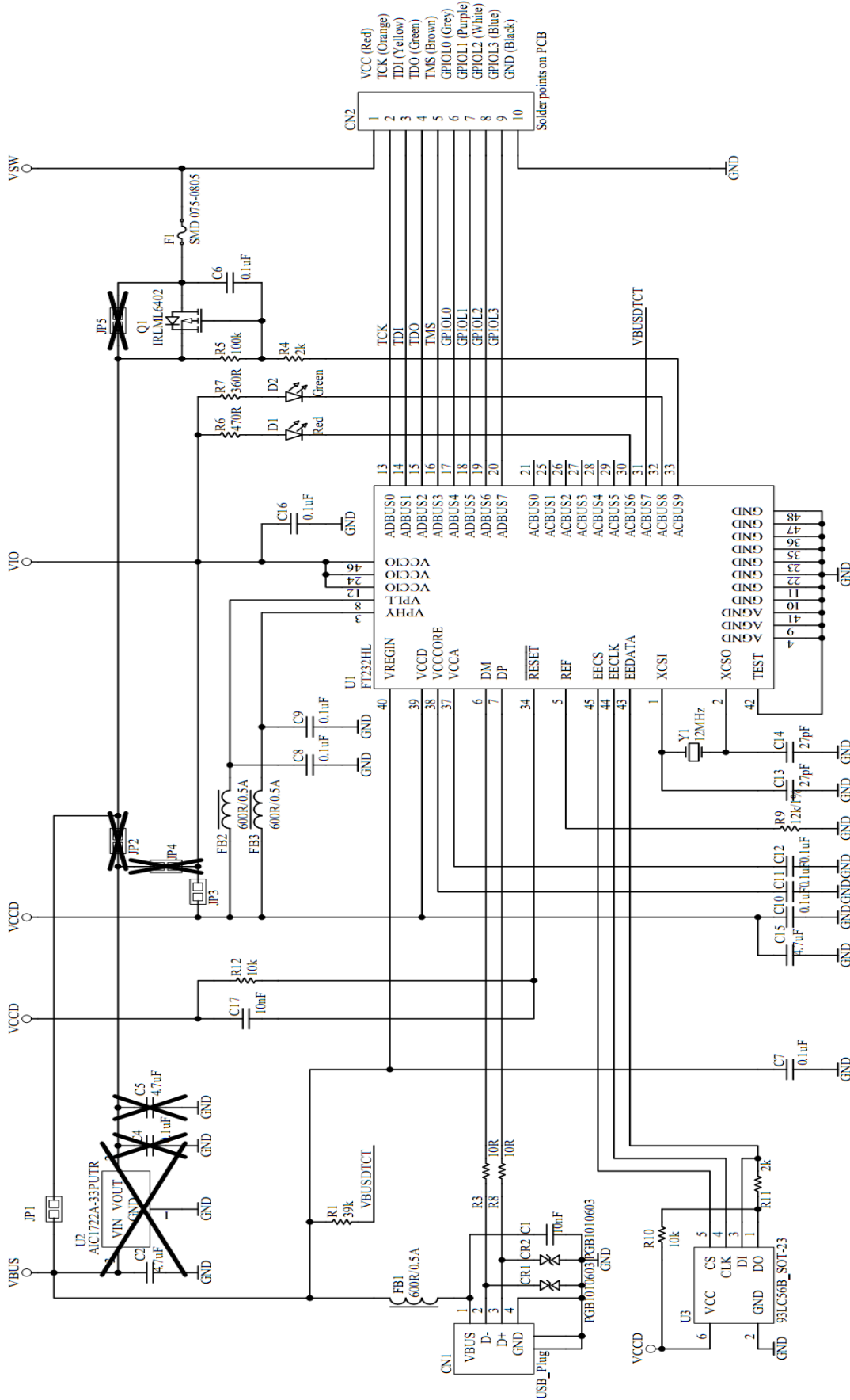
Figure 4-3 - Circuit Schematic of PCB - C232HD-EDHSP-0
