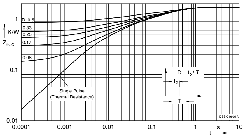
Fig. 6 Transient thermal impedance function to case at various duty cycles
