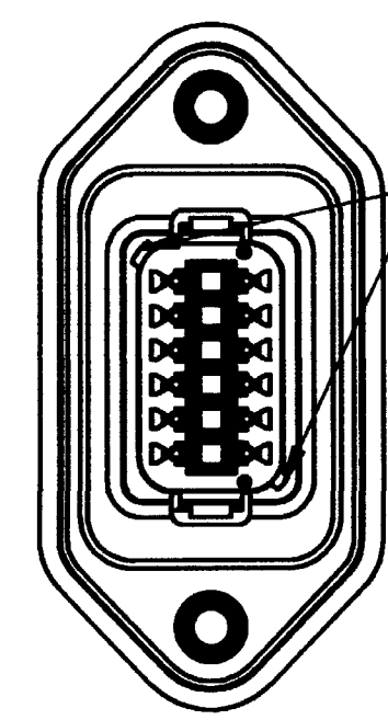
DT04-12PC-LE01 KEY ARR. -C- COLOR : GREEN (SHELL AND WELD CAP)
