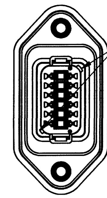
DT04-12PD-LE01 KEY ARR. -D- COLOR : BROWN (SHELL AND WELD CAP)
