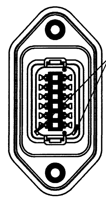
DT04-12PB-LE01 KEY ARR. -B- COLOR : BLACK (SHELL AND WELD CAP)
